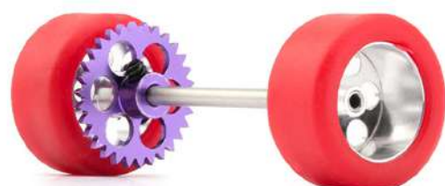
KIT RACING ULTRALIGHT RTR - Ø 15,8MM WHEELS 9132 FOR NSR CLASSIC CARS
